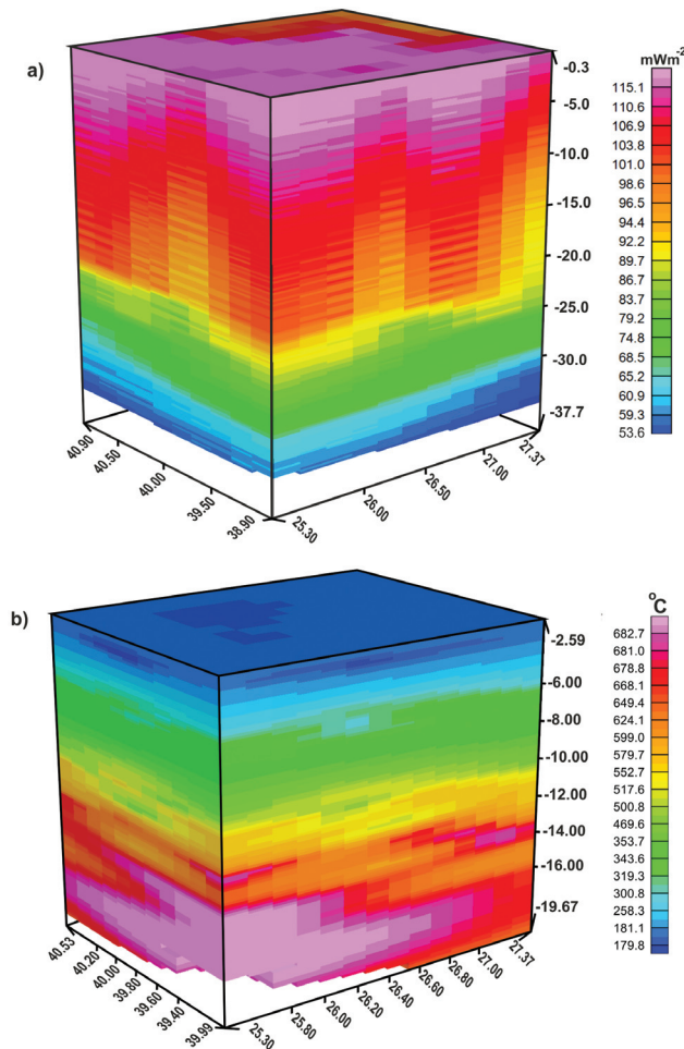
Fig. 9 3D block diagram representations: a) 3D heat flow and b) 3D temperature map of study area
