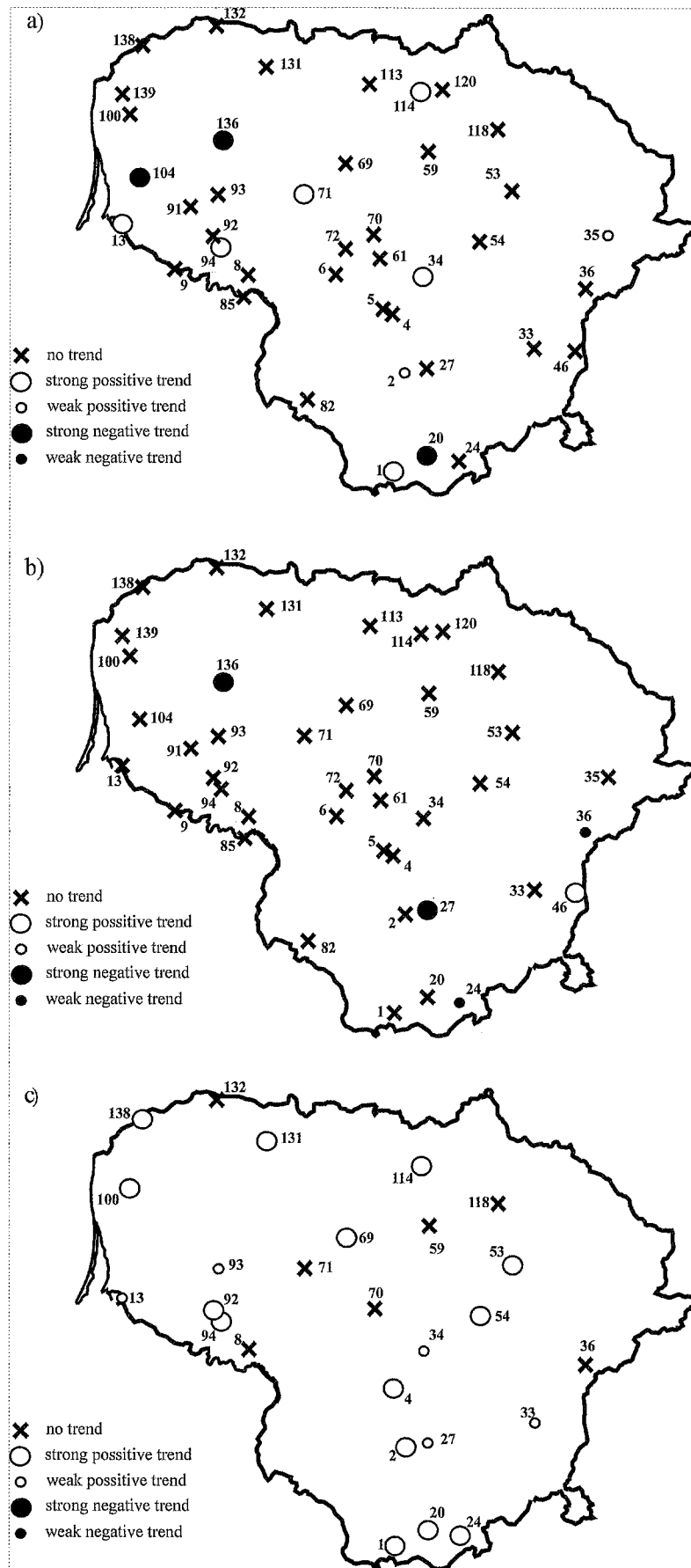
Fig. 5 Trends in river water temperature for the studied periods: a – the whole period, b – 1960-1991, c – 1991-2010. Compiled by D. Šarauskienė.
