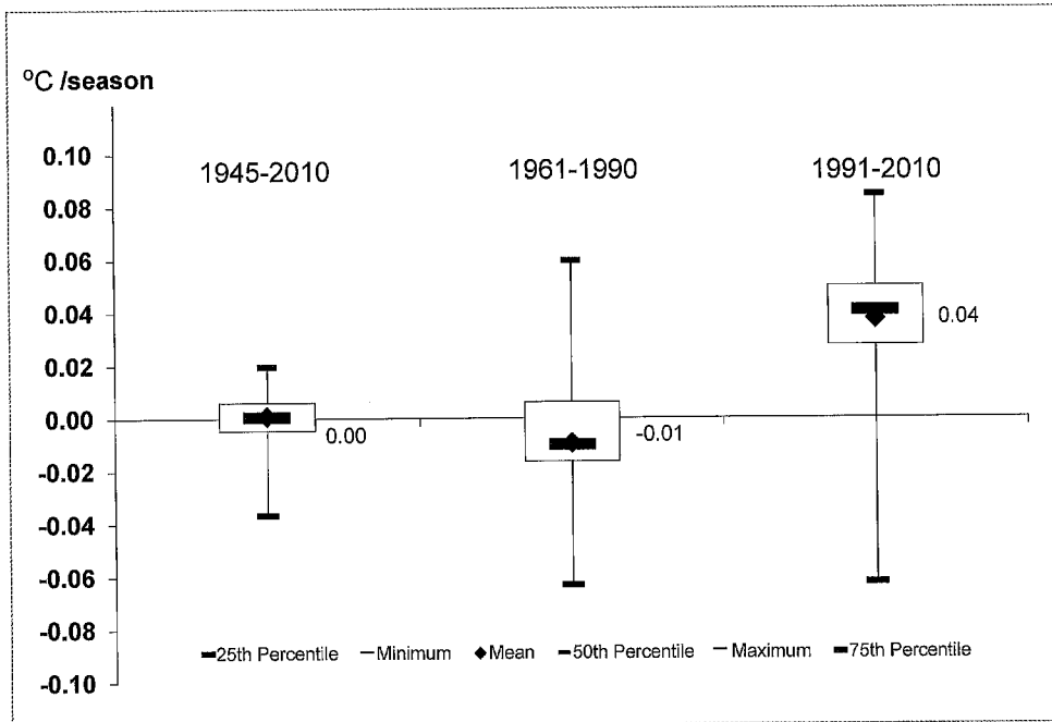
Fig. 6 Changes of slope of water temperatures for three studied periods. Compiled by J. Kriauciūnienė.
