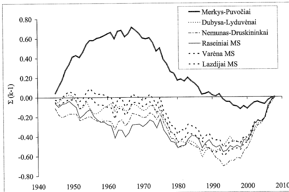
Fig. 7 The integral curves of variation of air and river water temperature of the warm season (May-October) in 1945-2010. Compiled by J. Kriauciūnienė.
