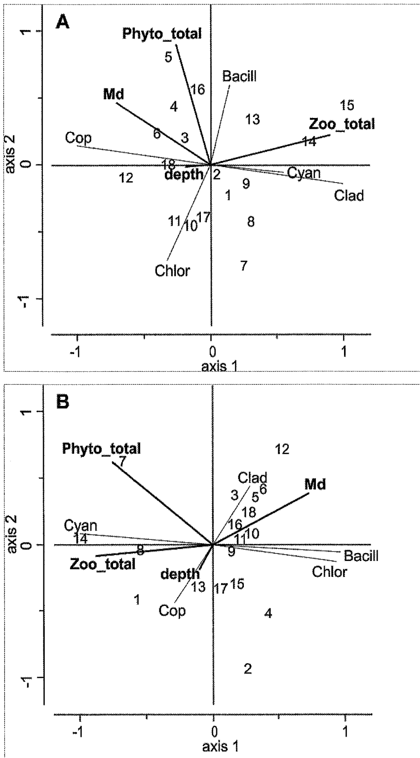
Fig. 7 RDA analysis for the river-lagoon transition at 18 July, 2001 (A) and 17 August, 2001 (B). Md – sediment median diameter; phyto_total – total abundance of phytoplankton; zoo_total – total abundance of zooplankton; Cyan – Cyanobacteria; Bacill – Bacillariophyceae; Chlor – Chlorophyceae; Cop – Copepoda; Clad – Cladocera. Compiled by Z.R. Gasiūnaitė and Š. Gulbinskas.
